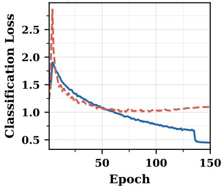
Training Loss Convergence — YOLOv8s v5 (Final), 150 Epochs
