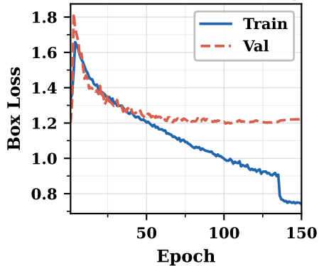
Training Loss Convergence — YOLOv8s v5 (Final), 150 Epochs
